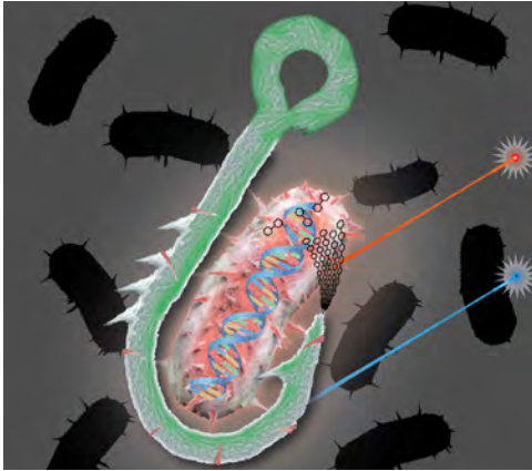
Graphical representation of the cellulose hook approach. (Devin Doud)
